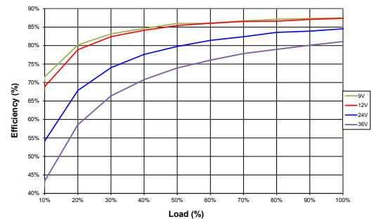
NCM6S1215C
