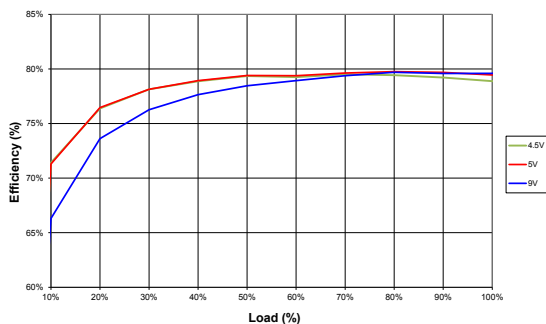
NCM6S0515C
