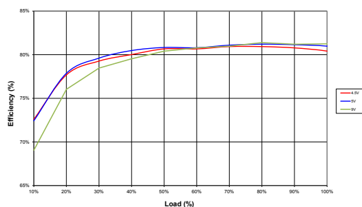
NCM6D0515C
