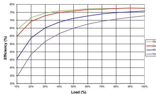
NCM6S4812C
