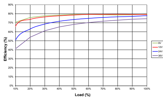
NCM6S1212C
