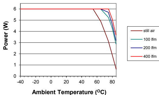
NCM6X4812C
