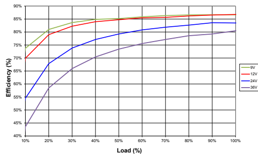
NCM6S1212C
