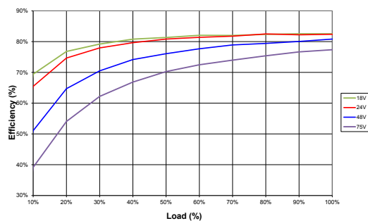
NCM6S4815C
