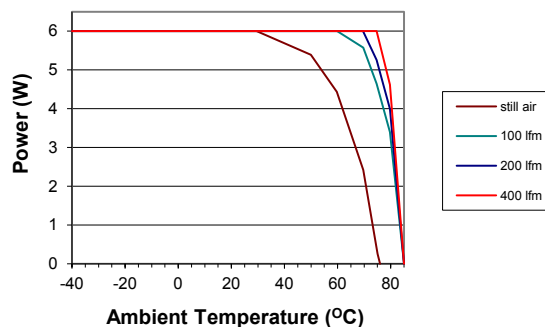
NCM6X4815C
