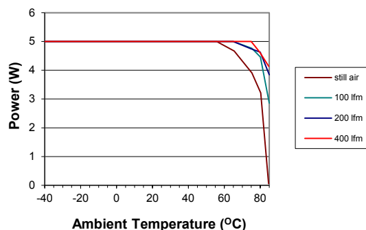
NCM6X0505C
