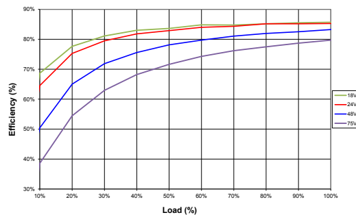
NCM6S4812C
