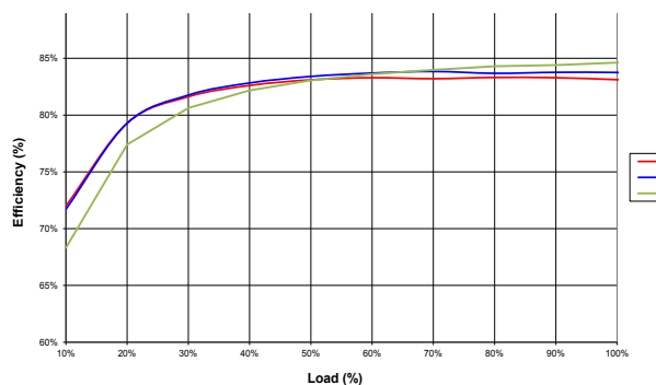
NCM6S0505C
