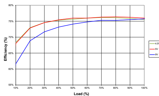
NCM6S0512C
