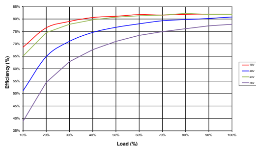
NCM6D4805C
