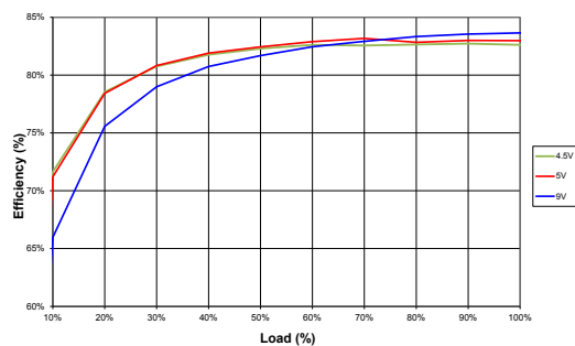
NCM6S0515C
