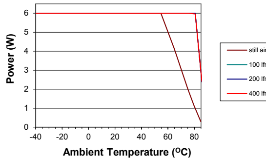
NCM6X4815C
