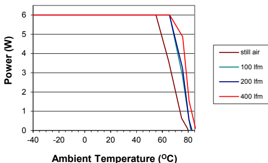
NCM6X1205C
