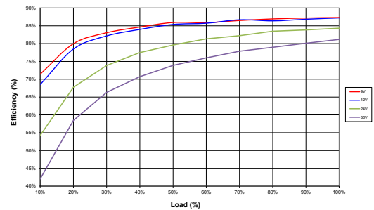
NCM6S1205C
