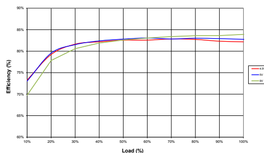
NCM6S0503C
