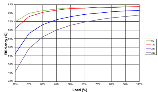
NCM6S1215C
