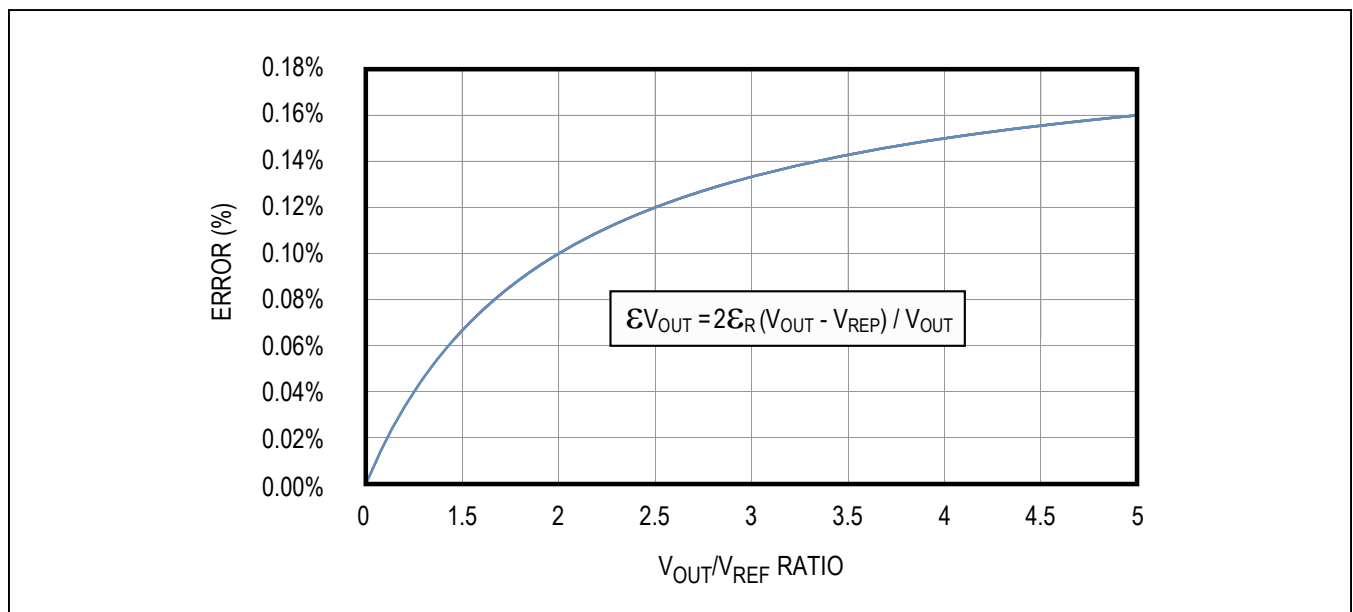
Figure 5. DC Accuracy Impact Showing Effect of 0.1% Tolerance for R_{FB1} and R_{FB2}
