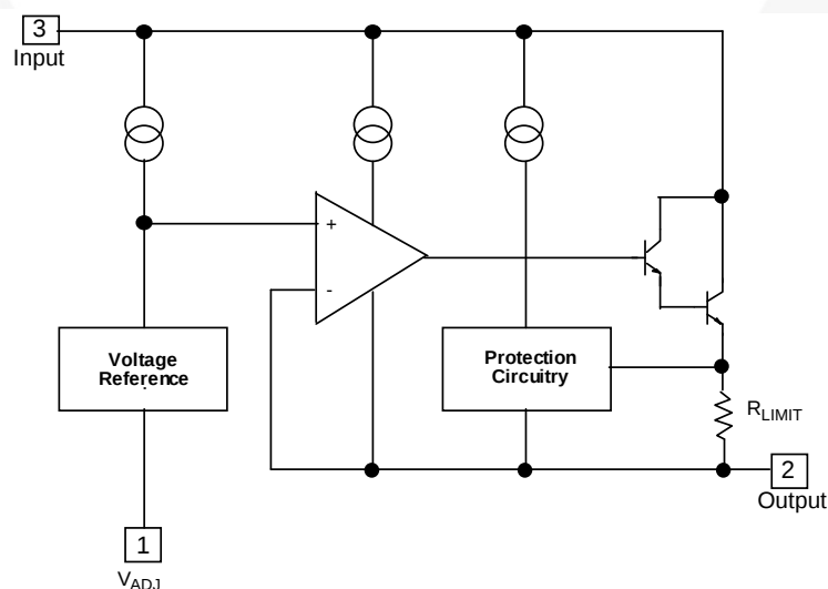
Figure 1. Block Diagram
