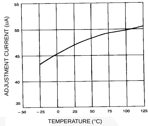
Figure 3. Adjustment Current
