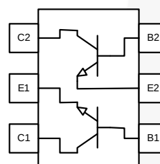
Figure 4. FMB2222A Internal Connection
