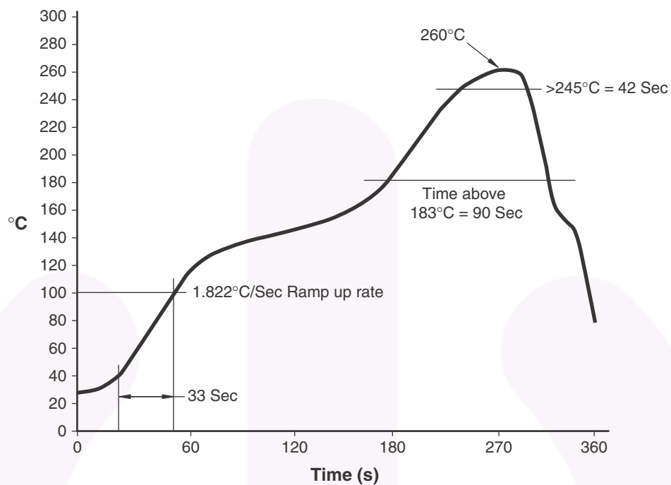
Figure 18. Reflow Profile
