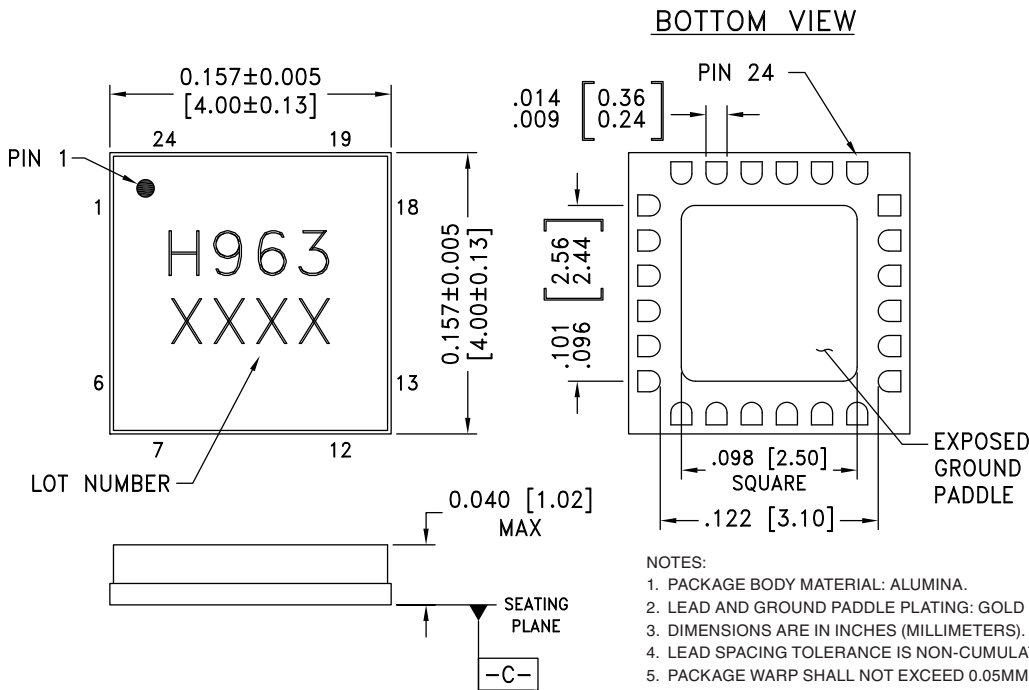
Outline Drawing
