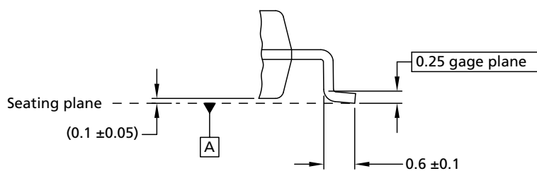
Detail A
