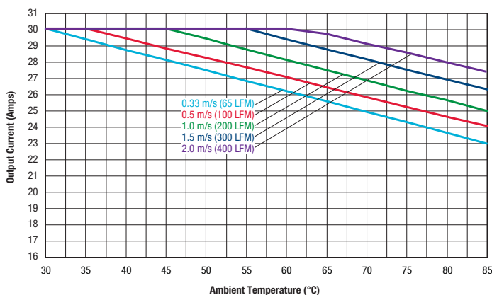
Maximum Current Temperature Derating @sea level (VIN = 24V, air flow from Pin 3 to Pin 1, with baseplate)
