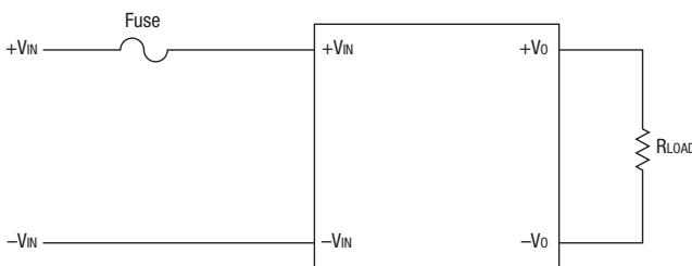
Figure 2. Input Fusing
