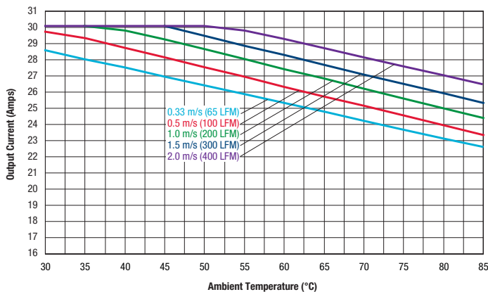
Maximum Current Temperature Derating @sea level (VIN = 48V, air flow from Pin 3 to Pin 1, with baseplate)
