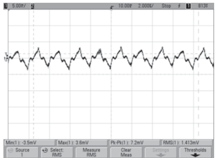
Output Ripple and noise (VIN = 48V, Vout = nom, Iout = 0A, Cloud = 330uF, Ta = +25°C)
