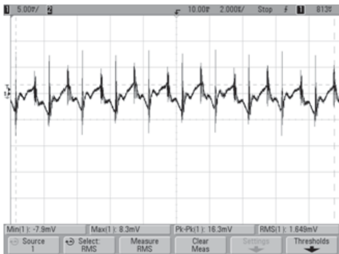
Output Ripple and noise (VIN = 48V, Vout = nom, Iout = 20A, Cloud = 330uF, Ta = +25°C)
