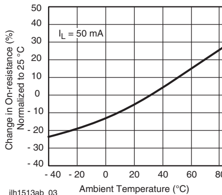
Fig. 4 - On-Resistance vs. Temperature
