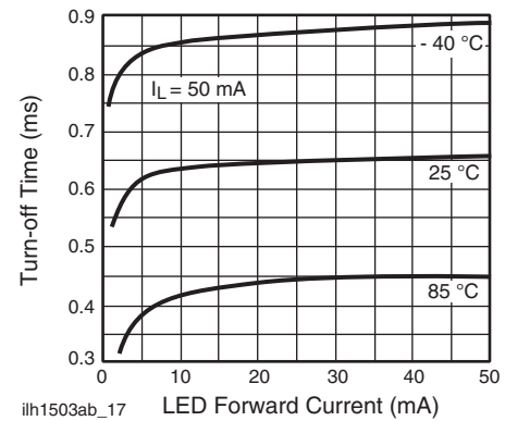
Fig. 18 - Turn-off Time vs. Temperature
