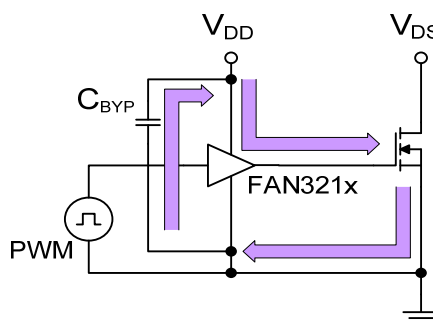
Figure 32. Current Path for MOSFET Turn-On
