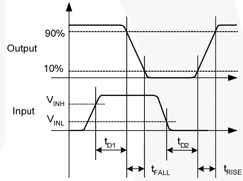
Figure 9. Inverting Timing Diagram
