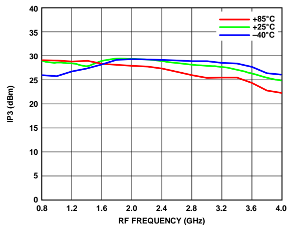
Figure 8. Output IP3 vs. RF Frequency over Temperature, Upper Sideband
