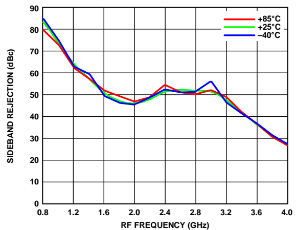
Figure 7. Sideband Rejection vs. RF Frequency over Temperature, Upper Sideband
