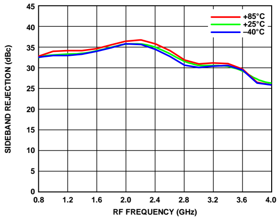
Figure 4. Sideband Rejection vs. RF Frequency over Temperature, Lower Sideband
