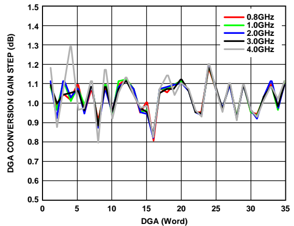
Figure 32. Conversion Gain Step vs. DGA Word over RF Frequency
