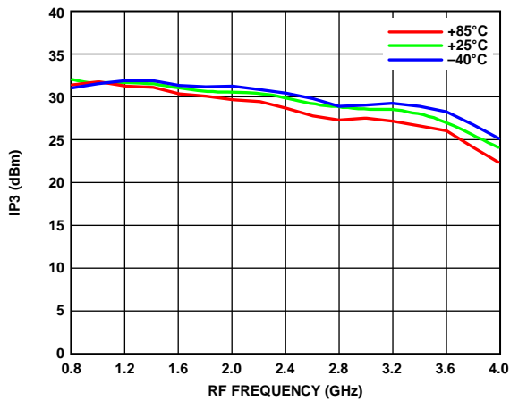
Figure 5. Output IP3 vs. RF Frequency over Temperature, Lower Sideband
