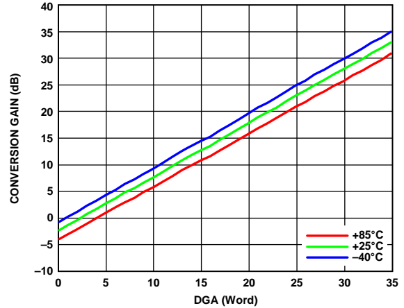
Figure 31. Conversion Gain vs. DGA Word over Temperature, Measurement Conducted with VCC_VGA = 3.3 V (Maximum Gain) on RF VGA, RF = 2 GHz
