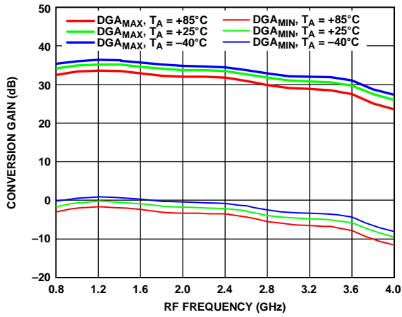
Figure 3. Conversion Gain vs. RF Frequency over Temperature, Lower Sideband
