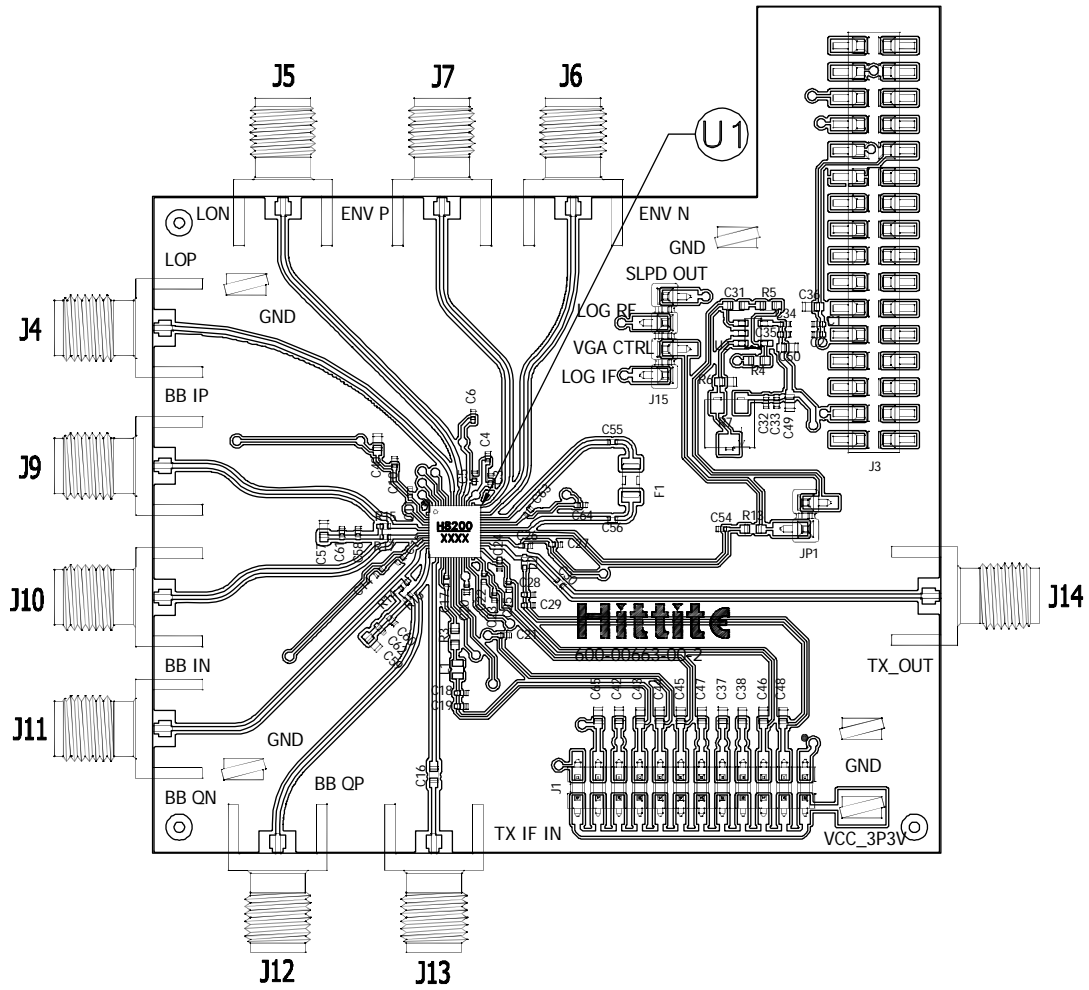
Figure 63. Evaluation PCB
