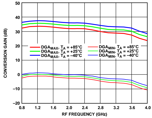
Figure 6. Conversion Gain vs. RF Frequency over Temperature, Upper Sideband
