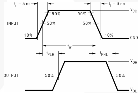
Figure 5. AC Waveforms
