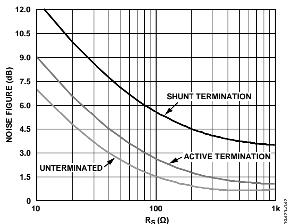
Figure 48. Noise Figure vs. R_S for Shunt Termination, Active Termination Matched and Unterminated Inputs, V_{\text{GAIN}} = 1.6\ \text{V}
