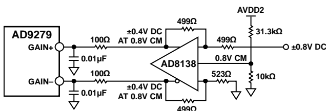
Figure 52. Differential GAIN± Pin Configuration
