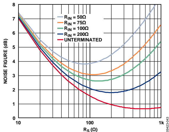
Figure 49. Noise Figure vs. R_S for Various Fixed Values of R_{IN} , Active Termination Matched Inputs, V_{\text{GAIN}} = 1.6\ \text{V}
