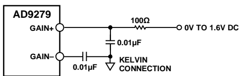
Figure 51. Single-Ended GAIN± Pin Configuration
