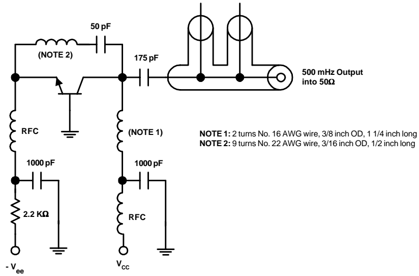
FIGURE 1: 500 MHz Oscillator Circuit
