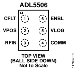
Figure 2. Pin Configuration
