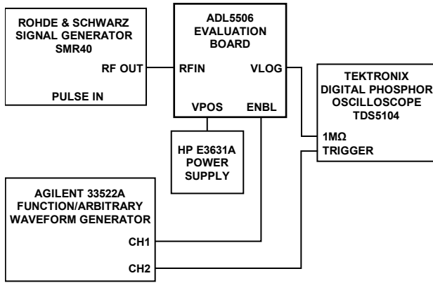
Figure 39. Hardware Configuration for Output Response to ENBL Pin Gating Measurements
