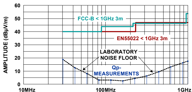
FIGURE 7. UNDETECTABLE EMISSIONS OF GMR ISOLATORS
