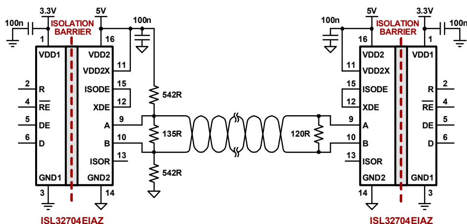
FIGURE 1. TYPICAL ISOLATED HIGH-SPEED RS-485 APPLICATION
