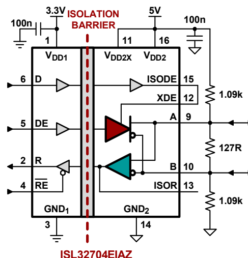
FIGURE 10. TYPICAL OSOP TRANSCIEVER CONNECTIONS
