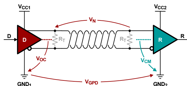
FIGURE 3. COMMON-MODE VOLTAGES IN A NON-ISOLATED DATA LINK
