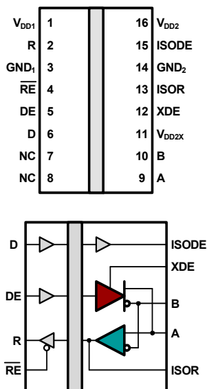
ISL32704E (16 LD QSOP) TOP VIEW
