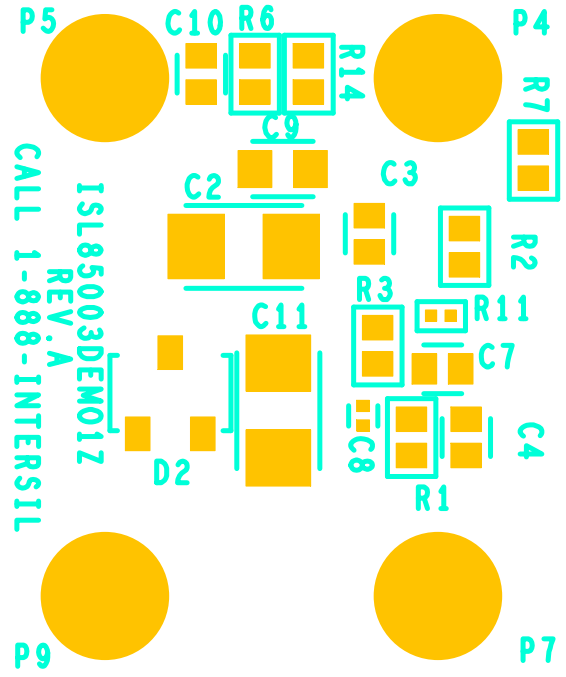
FIGURE 3. SILK SCREEN BOTTOM
