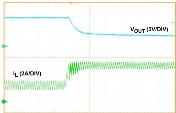
FIGURE 39. HIGH-SIDE FORWARD OVER CURRENT PROTECTION
