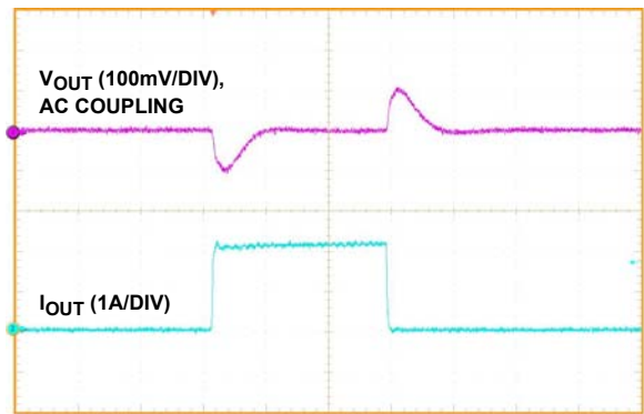
FIGURE 37. LOAD TRANSIENT, 0A \rightarrow 2.5A \rightarrow 0A , 2.5A/\mu s
