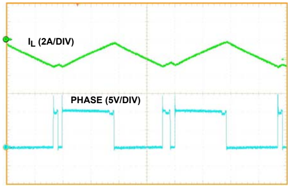
FIGURE 41. LOW-SIDE MOSFET REVERSE OVER CURRENT PROTECTION
