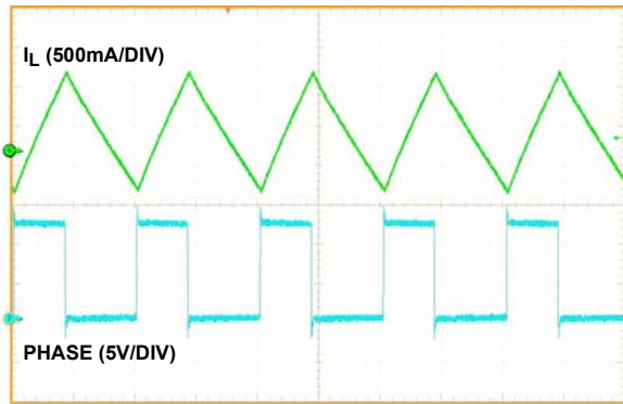
FIGURE 36. STEADY STATE IN FORCED CCM, I_{OUT} = 0.2A
