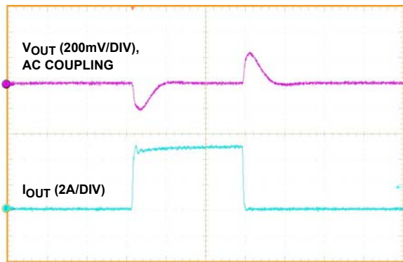
FIGURE 38. LOAD TRANSIENT, 0A \rightarrow 5A \rightarrow 0A , 2.5A/\mu s
