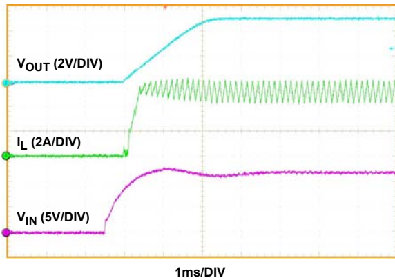
FIGURE 30. START-UP WITH V_{IN} , I_{OUT} = 5A
