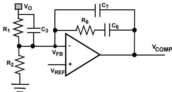
FIGURE 47. TYPE II COMPENSATOR
