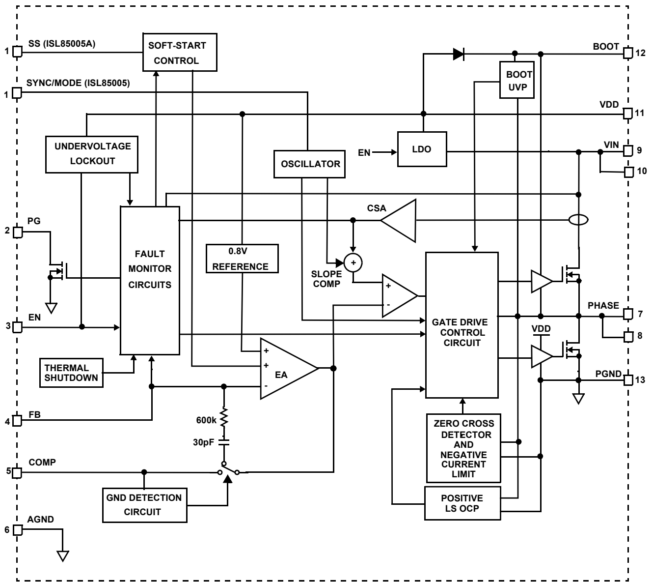
FIGURE 3. BLOCK DIAGRAM
