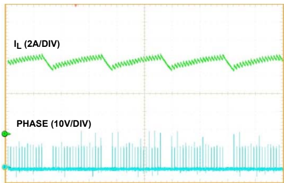
FIGURE 40. OUTPUT SHORT-CIRCUIT BEHAVIOR
