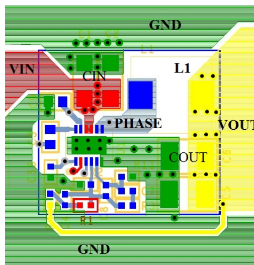
FIGURE 49. RECOMMEND LAYOUT (TOP LAYER)
