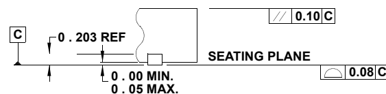
DETAIL "X"
