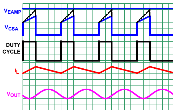
FIGURE 42. CCM OPERATION WAVEFORMS
