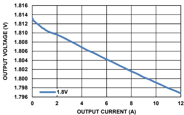
FIGURE 8. V_{OUT} REGULATION vs LOAD ( V_{IN} = 12V , CCM, 600kHz)
