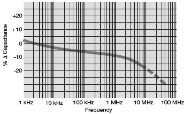
Δ Capacitance vs. Frequency
