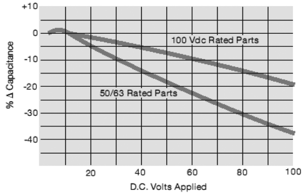
Voltage Coefficient
