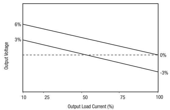
CRE1S1212SC
