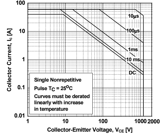
Figure 10. SOA Characteristics
