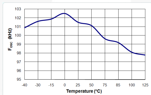
Figure 16. f osc vs. Temperature
