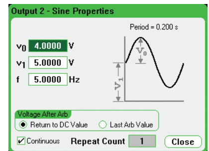
Figure 8. Once you have selected a waveform, you simply fill in the blanks to describe the waveform.
