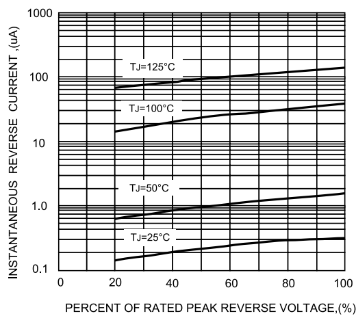
FIG.5-TYPICAL REVERSE CHARACTERISTICS
