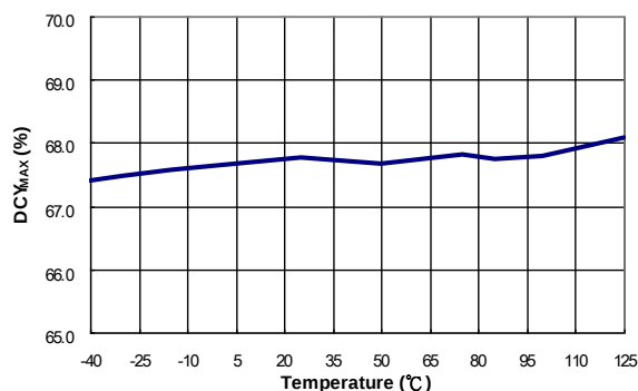
Figure 11. Maximum Duty Cycle ( DCY_{MAX} ) vs. Temperature
