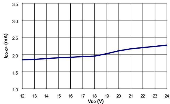
Figure 15. Operating Supply Current vs. V DD Voltage
