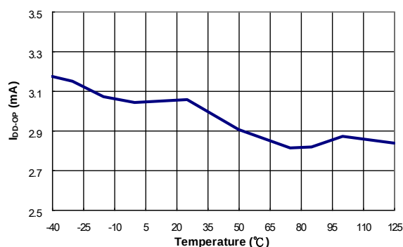
Figure 9. Operating Supply Current ( I_{DD-OP} ) vs. Temperature
