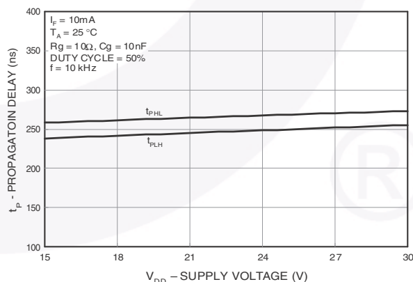
Fig. 14 Propagation Delay vs. Supply Voltage
