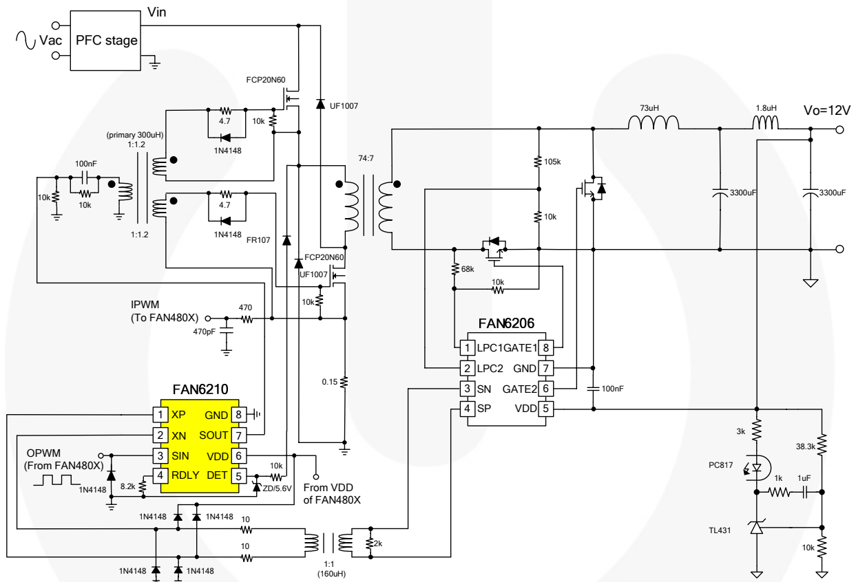
Figure 18. Application Circuit
