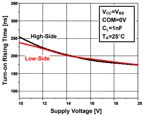
Figure 8. Turn-On Rising Time vs. Supply Voltage
