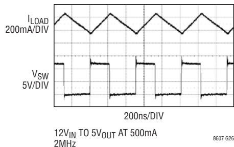
Switching Waveforms
