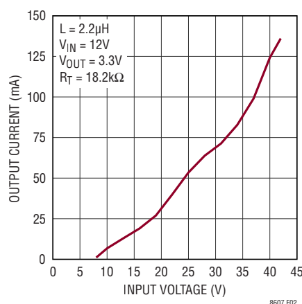
Figure 2. Minimum Load to Full Frequency (SYNC Float to 1.9V)
