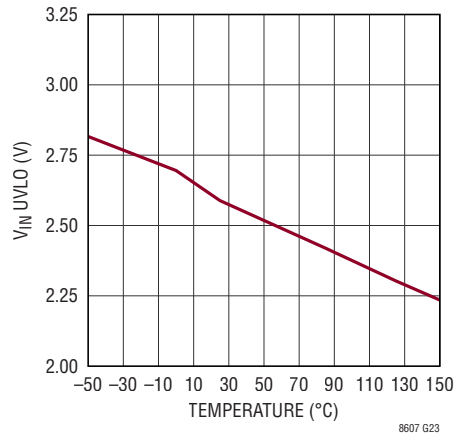
V IN UVLO vs Temperature
