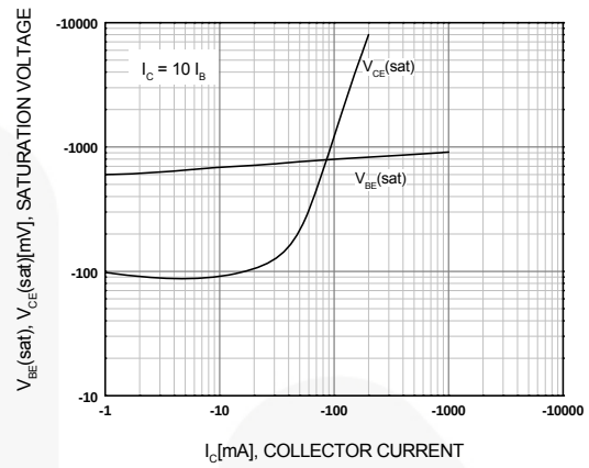
Figure 2. Base-Emitter Saturation Voltage and Collector-Emittor Saturation Voltage
