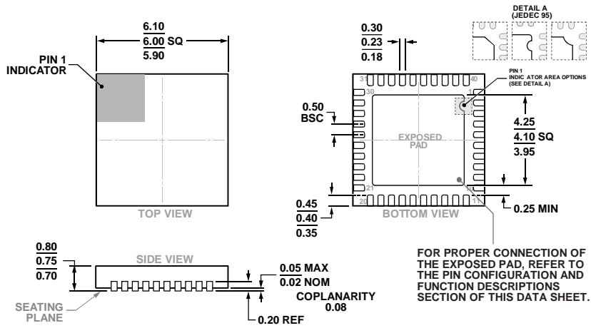
Figure 13. 40-Lead Lead Frame Chip Scale Package [LFCSP] 6 x 6 mm Body and 0.75 mm Package Height (CP-40-9) Dimensions shown in millimeters
