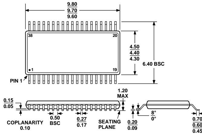
Figure 14. 38-Lead Thin Shrink Small Outline Package [TSSOP] (RU-38) Dimensions shown in millimeters
