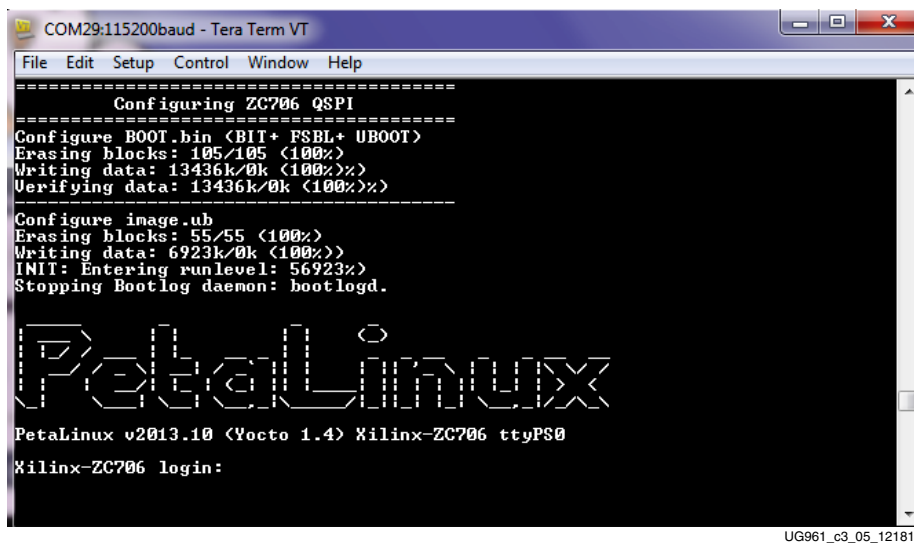
Figure 3-5: Initialization Progress of the init.sh Script
