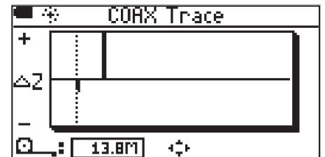
Figure 4. Run a coax TDR trace to see where large impedance changes are located.
