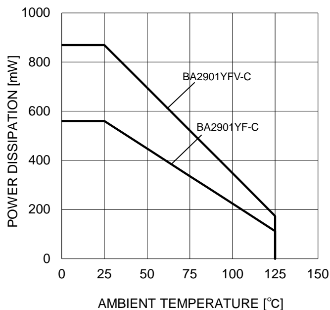
Figure 25. Derating Curve
