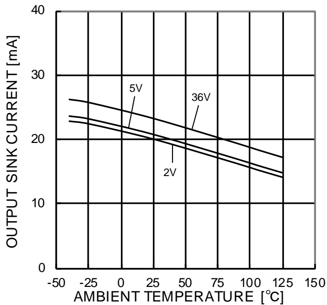
Figure 31. Output Sink Current – Ambient Temperature ( V_{OUT}=1.5V )
