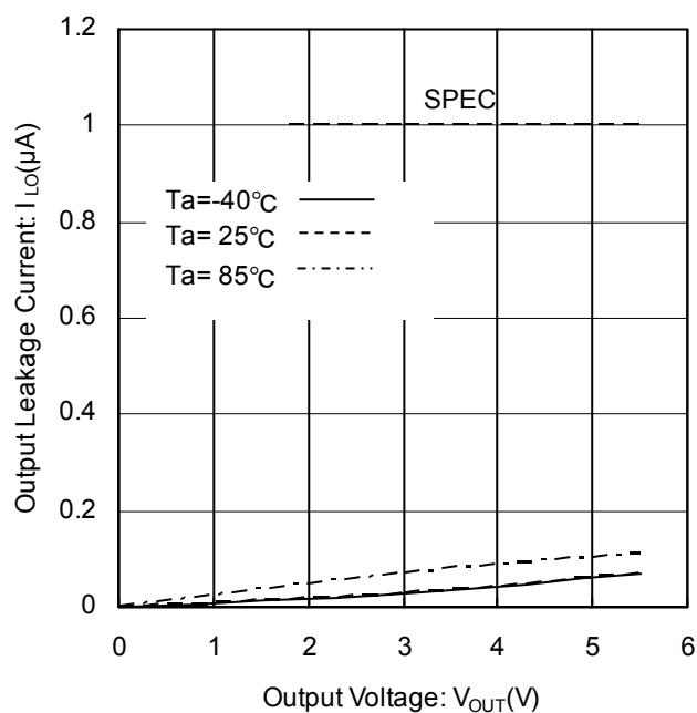
Figure 9. Output Leakage Current vs Output Voltage (SDA)
