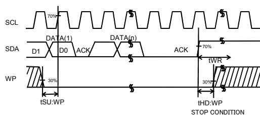
Figure 2-(d). WP Timing at Write Execution
