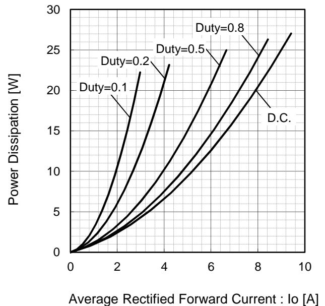
Fig.8 I_o - P_f Characteristics
