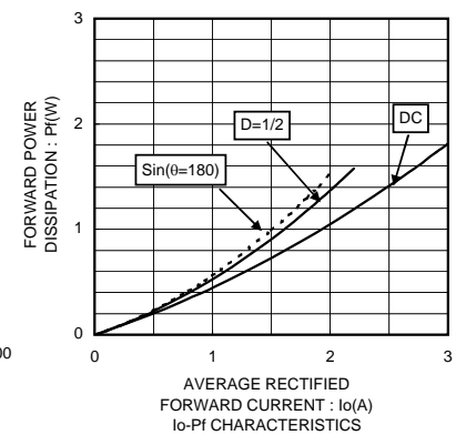
I_o - P_f CHARACTERISTICS
