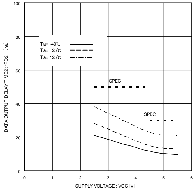
Figure 26. Data Output Delay Time t_{PD2} ( CL=30\text{pF} )
