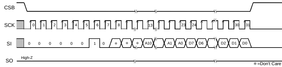
Figure 38. Write command
