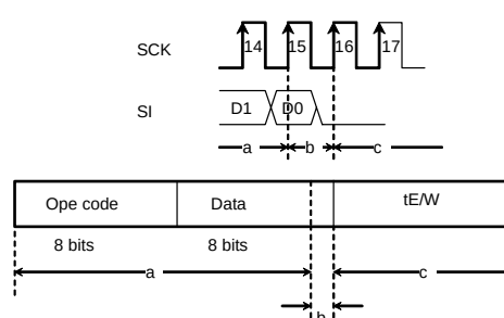
Figure 49. WRSR cancel valid timing
