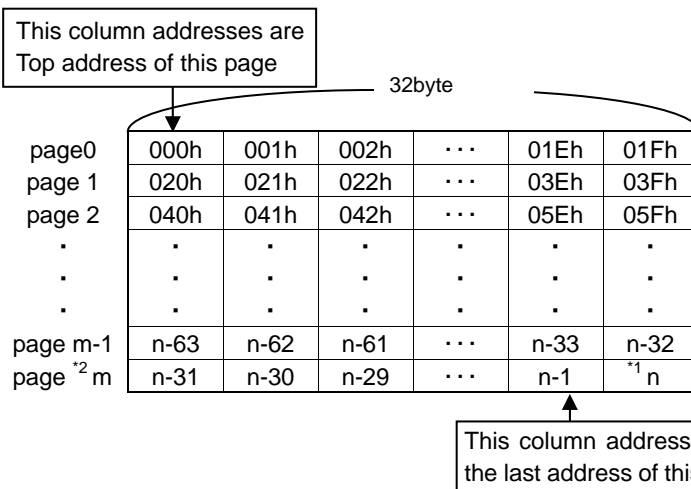
Figure 40. EEPROM physical address for Page write command (32Byte)
