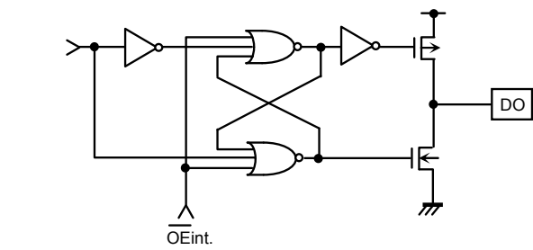
Figure 36 Output Circuit (DO)
