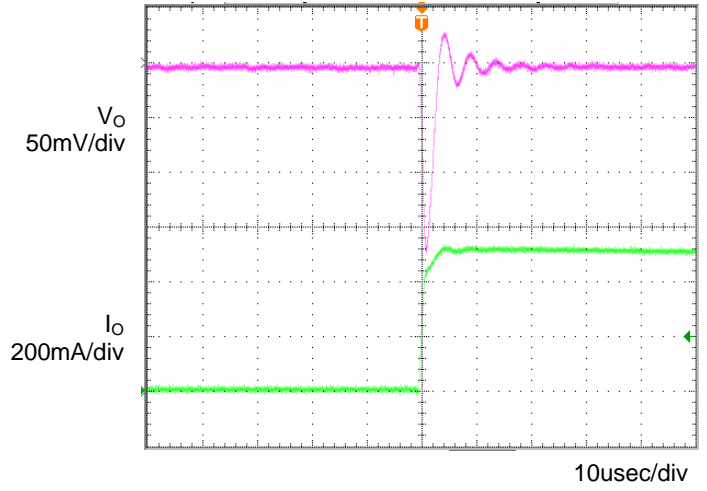
Fig.4 Transient Response (0→0.5A) C o =1μF, T a =25°C
