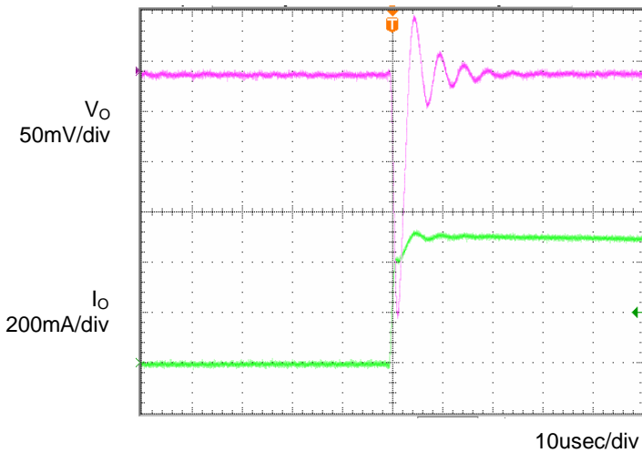
Fig.5 Transient Response (0→0.5A) C o =1μF, T a =105°C
