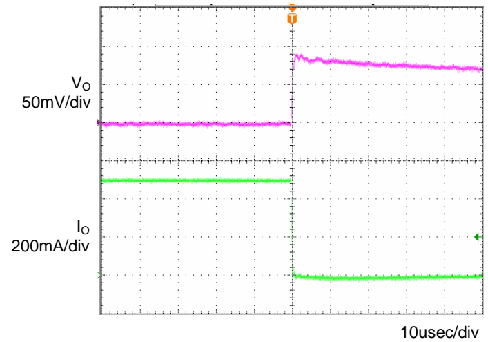
Fig.6 Transient Response (0.5→0A) C o =1μF, T a =-40°C
