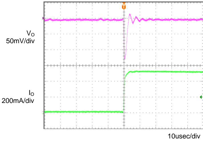
Fig.3 Transient Response (0→0.5A) C o =1μF, T a =-40°C
