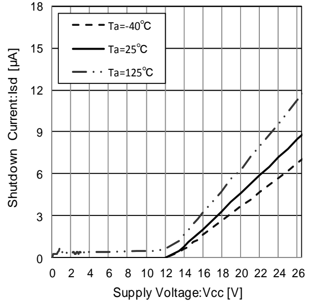
Figure 59. Shutdown Current
