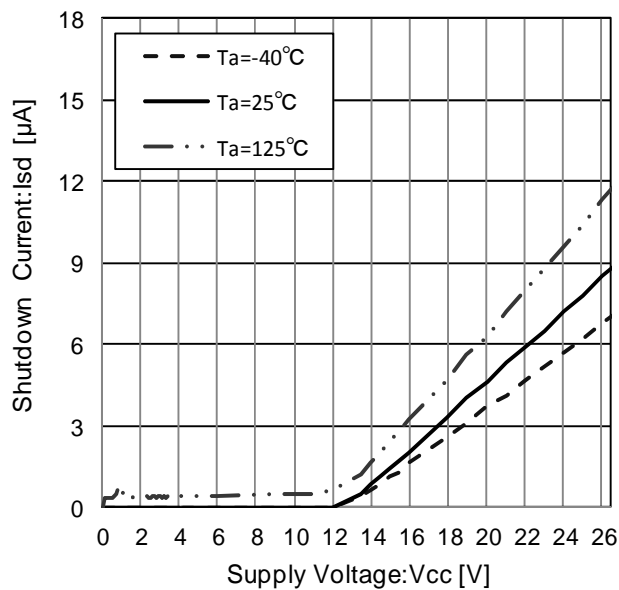
Figure 12. Shutdown Current
