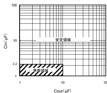
Cin vs Cout
