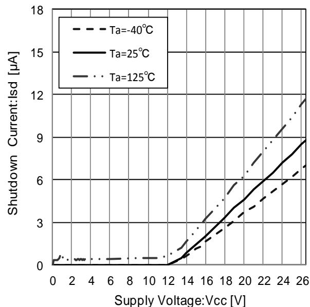
Figure 35. Shutdown Current
