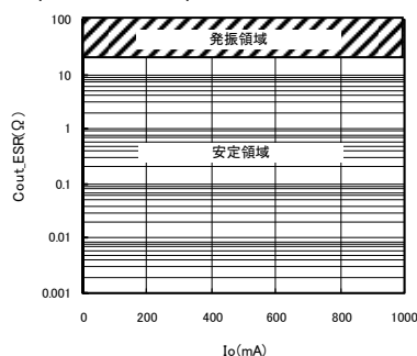
Cout_ESR vs Io 1.0V \leq V_O < 3.0V
