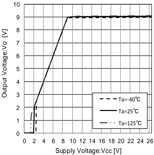
Figure 60. Line Regulation (Io=0mA)
