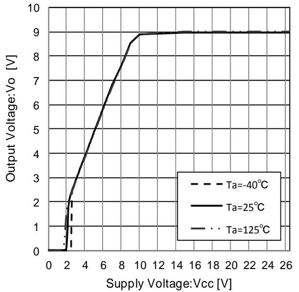
Figure 61. Line Regulation (Io=500mA)
