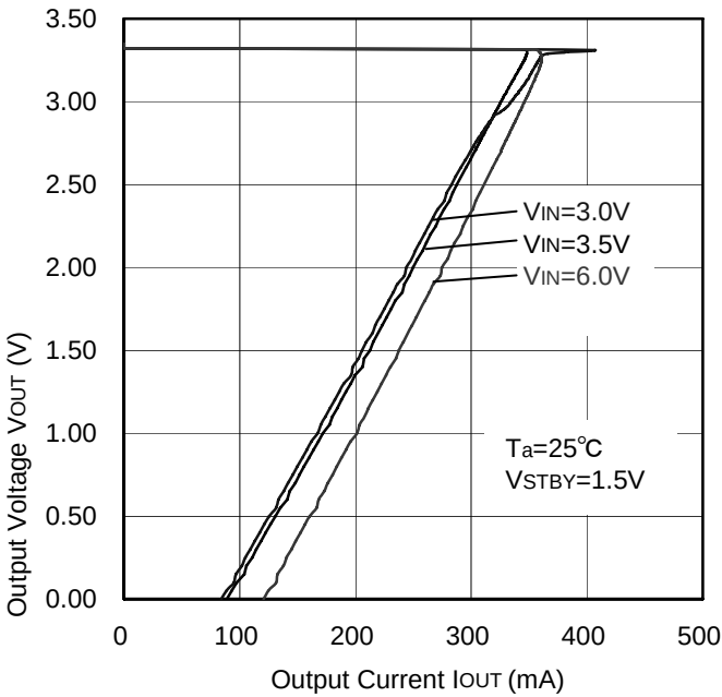
Figure 75. OCP Threshold
