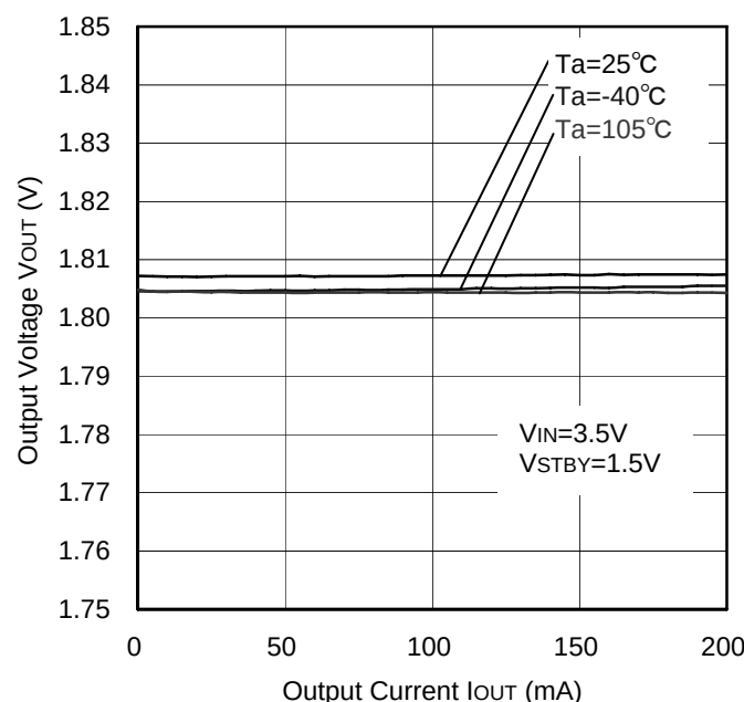
Figure 28. Load Regulation
