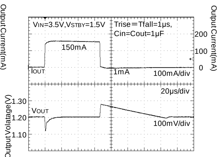
Figure 18. Load Response (1mA to 150mA)
