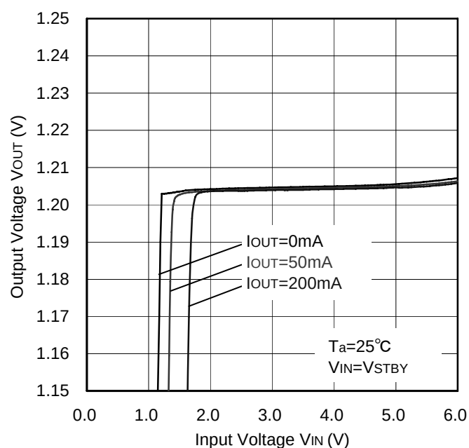
Figure 4. Line Regulation
