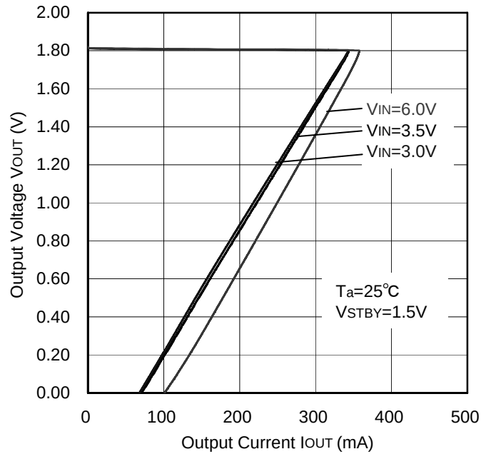
Figure 30. OCP Threshold
