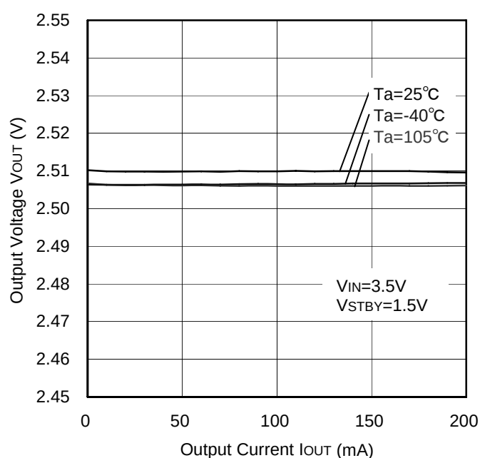
Figure 50. Load Regulation
