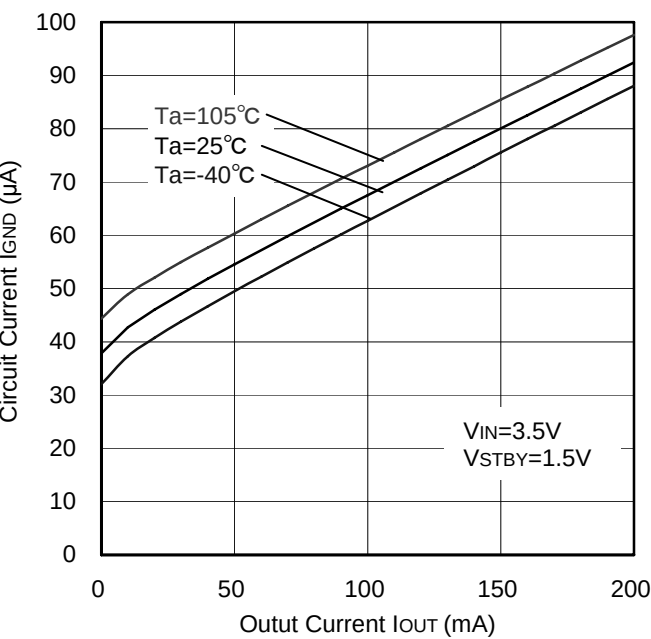
Figure 51. Circuit Current vs. Output Current
