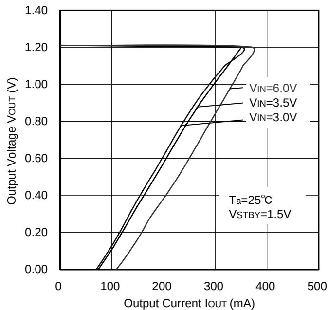
Figure 8. OCP Threshold
