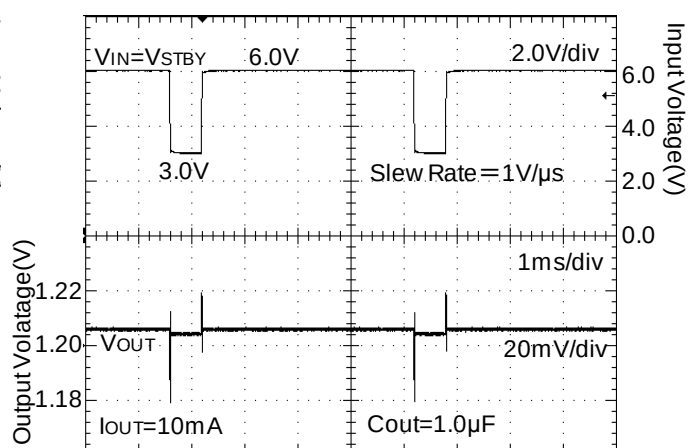
Figure 20. Line Transient Response (3.0 to 6.0V)
