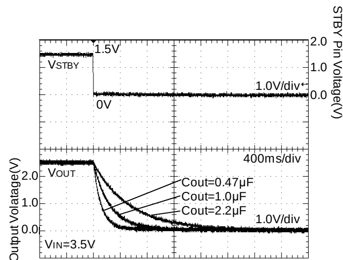
Figure 68. Discharge Time (ROUT=none)
