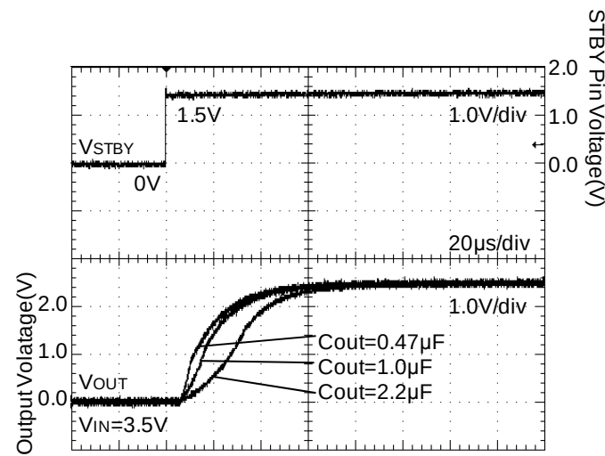
Figure 66. Startup Time (ROUT=none)
