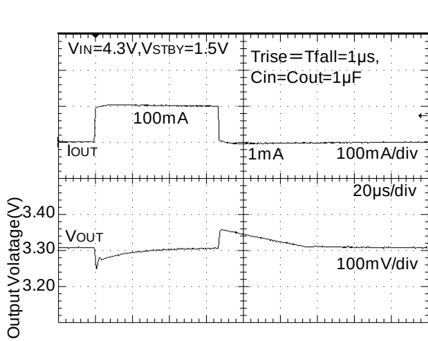
Figure 85. Load Response (1mA to 100mA)
