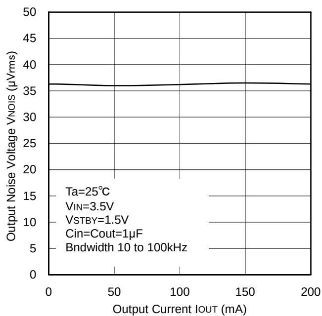
Figure 60. Output Noise Voltage vs. Output Current
