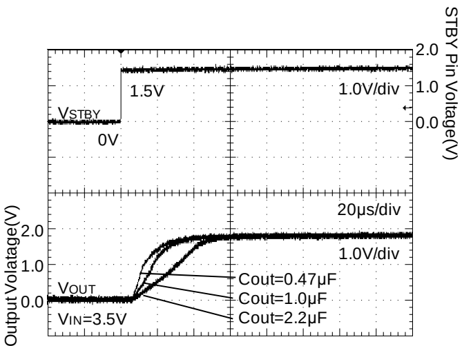
Figure 44. Startup Time (ROUT=9Ω)
