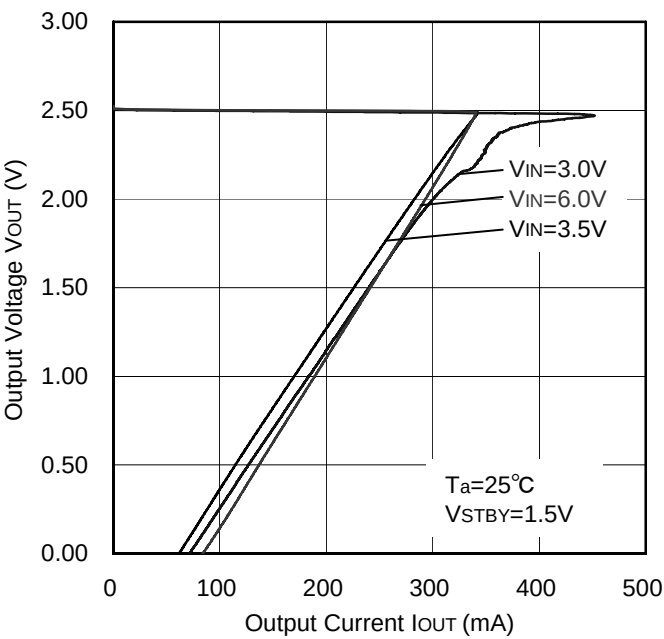
Figure 52. OCP Threshold
