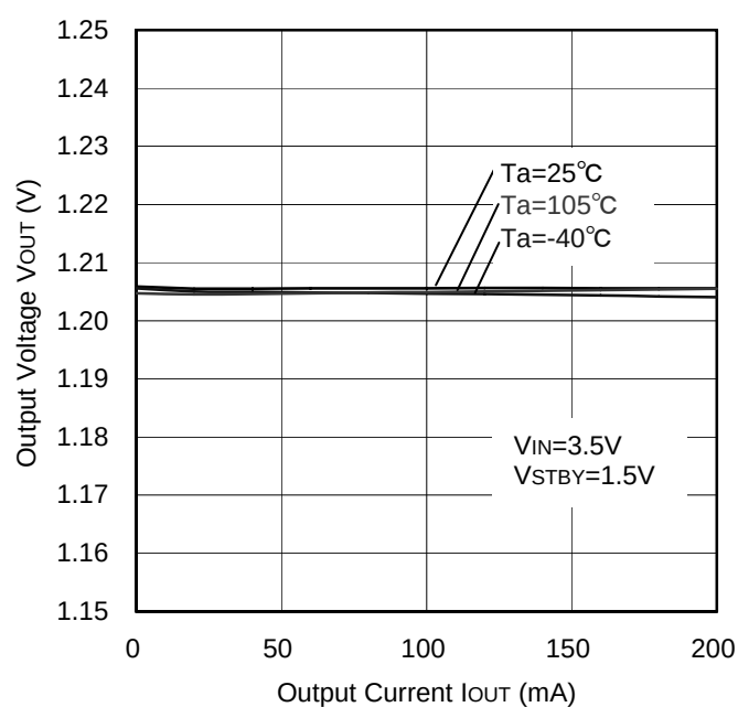
Figure 6. Load Regulation
