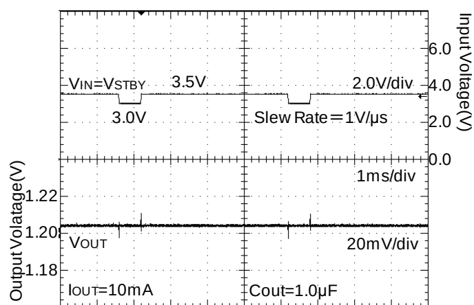
Figure 19. Line Transient Response (3.0 to 3.5V)
