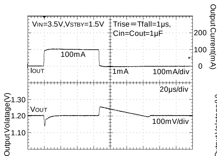
Figure 17. Load Response (1mA to 100mA)
