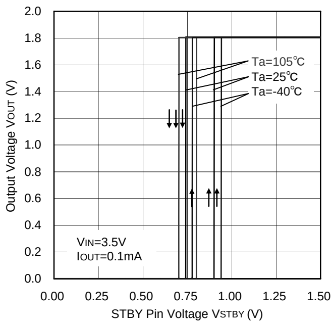
Figure 33. STBY Threshold
