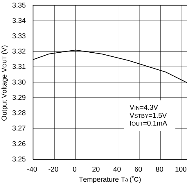
Figure 76. Output Voltage vs. Temperature
