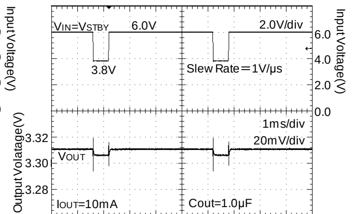
Figure 88. Line Transient Response (3.8 to 6.0V)
