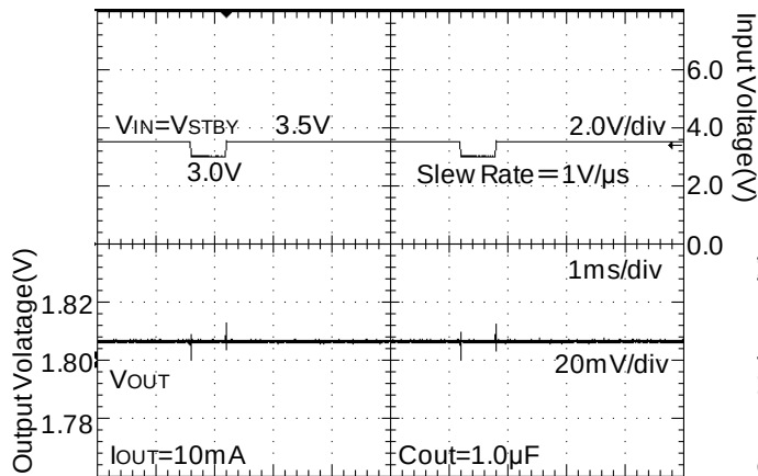
Figure 41. Line Transient Response (3.0 to 3.5V)
