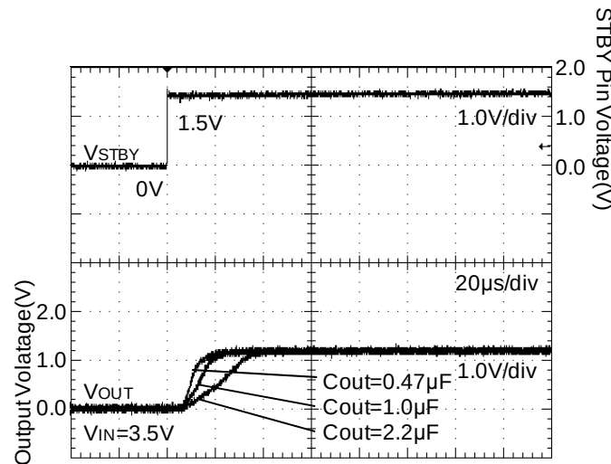
Figure 22. Startup Time (ROUT=6Ω)
