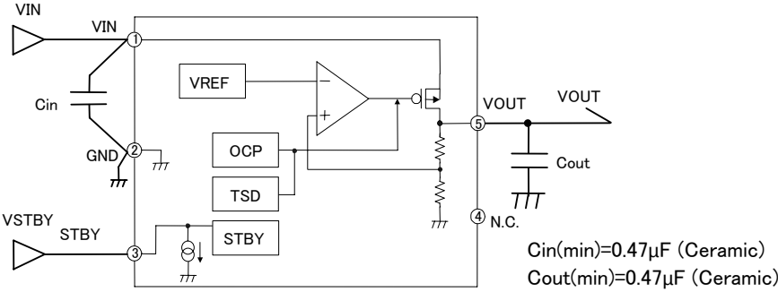
Figure 2. Block diagram
