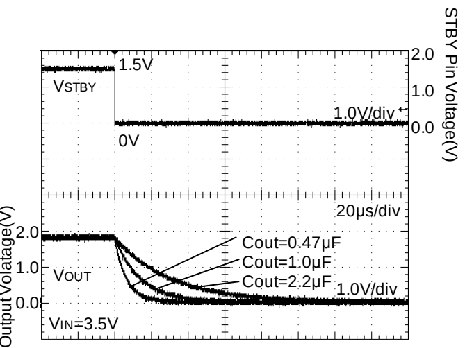
Figure 46. Discharge Time (ROUT=9Ω)
