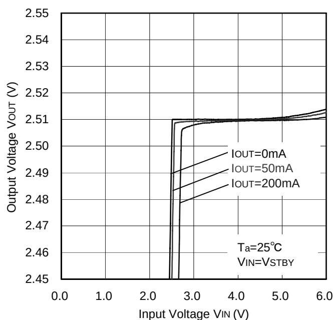
Figure 48. Line Regulation
