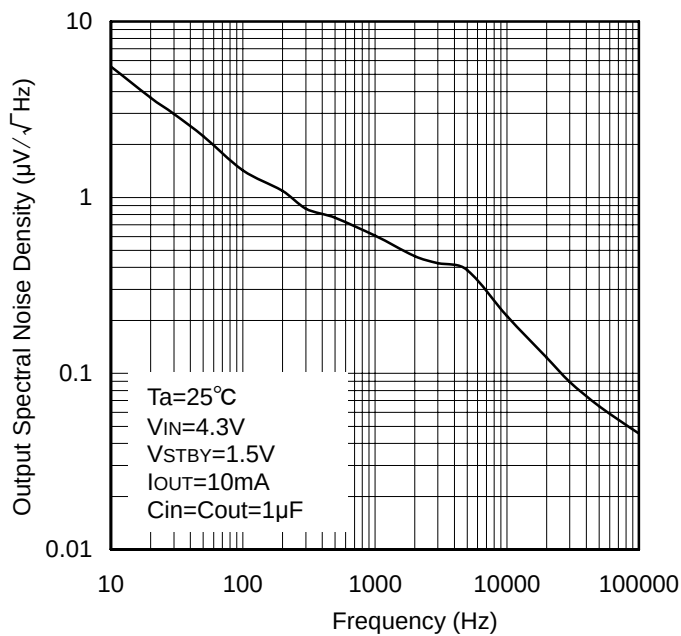
Figure 84. Output Spectral Noise Density vs. Frequency
