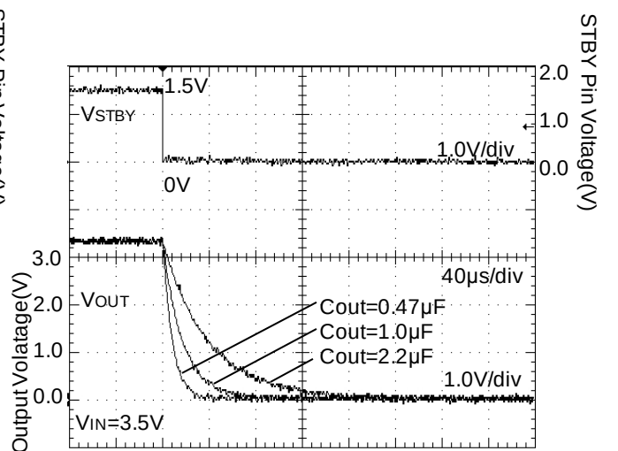
Figure 92. Discharge Time (ROUT=16.5Ω)
