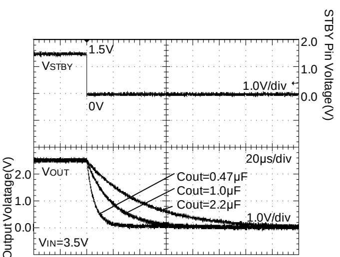
Figure 69. Discharge Time (ROUT=12.5Ω)
