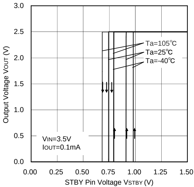
Figure 55. STBY Threshold
