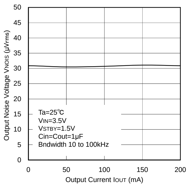
Figure 37. Output Noise Voltage vs. Output Current
