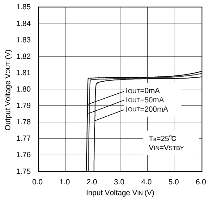
Figure 26. Line Regulation
