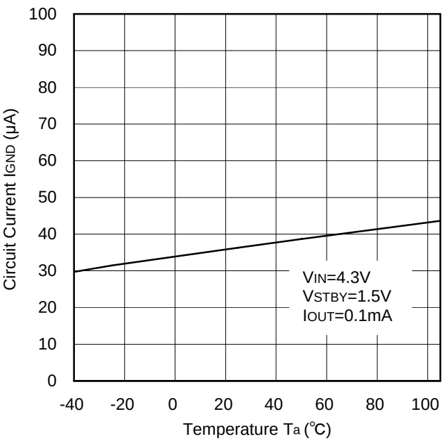
Figure 77. Circuit Current vs. Temperature
