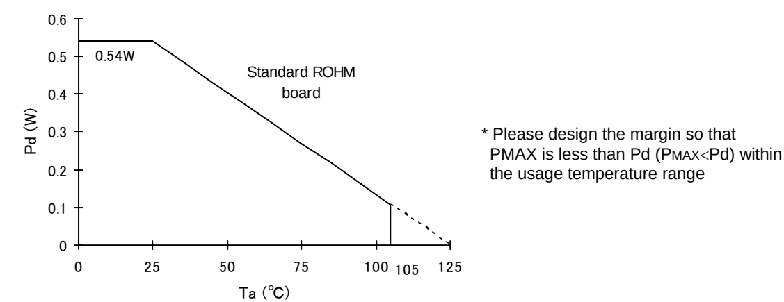
Figure 95. SSOP5 Power dissipation heat reduction characteristics (Reference)
